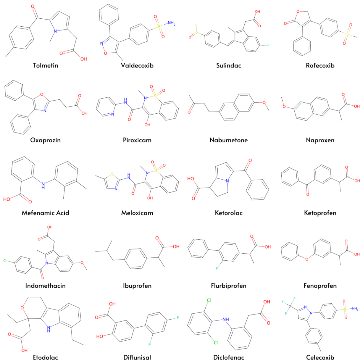
Figure S1. 2D illustration of retrieved anti-inflammatory drugs from the PubChem database
